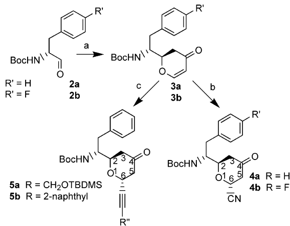
Scheme 2. Reagents and conditions: (a) \text{CH}_2=\text{C}(\text{OSiMe}_3)\text{CH}=\text{CHOMe} , \text{LiClO}_4 , \text{Et}_2\text{O} , rt; (b) \text{TMSCN} , \text{BF}_3\text{Et}_2\text{O} , \text{DCM} , 0^\circ\text{C} ; (c) \text{R}-\text{C}\equiv\text{CH} , \text{BuLi} , \text{TMSI} , \text{CuI}^*\text{DMS} , \text{THF} .
