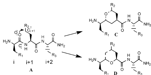
Chart 1. Design of tetrahydropyran analogues using C_i' = O_i' \cdots C_{i+1}' mode of peptide bridging.
