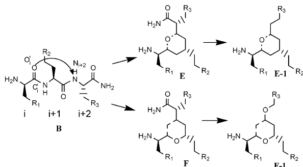
Chart 2. Design of tetrahydropyran analogues using C_i' = O_i' \cdots N_{i+2} mode of peptide bridging.
