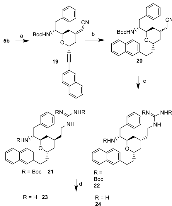
Scheme 5. Reagents and conditions: (a) (EtO) 2 OPCH 2 CN, NaH, THF, −40 °C; (b) H 2 , 40PSI, Wilkinson cat., toluene; (c) (i) H 2 , Ni/Ra, MeOH/NH 4 OH (1:4); (ii) BocHNC(=NBoc)SMe, HgCl 2 , Et 3 N, DMF, 0 °C; (d) TFA, DCM.
