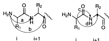
Scheme 1. Examples of frequently used modes of conceptual bridging atoms in dipeptide moieties leading to cyclic peptidomimetics. Modes of bridging: a. N_i-N_{i+1} ; b. N_i-C_{i+1}'N_i-C_i^{\gamma} ; c. C_i^{\gamma}-N_{i+1} ; d. C_i^{\gamma}-C_{i+1}^{\gamma} .
